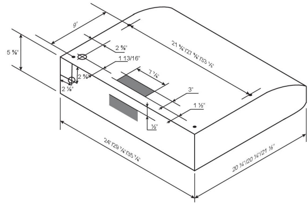
ISOMETRIC
