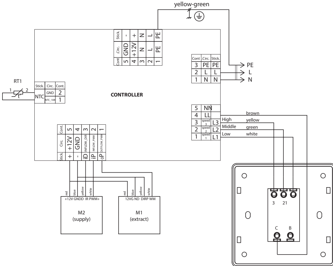
WIRING DIAGRAM FOR THE UNIT WITH SP3-1 SENSOR SPEED SWITCH
